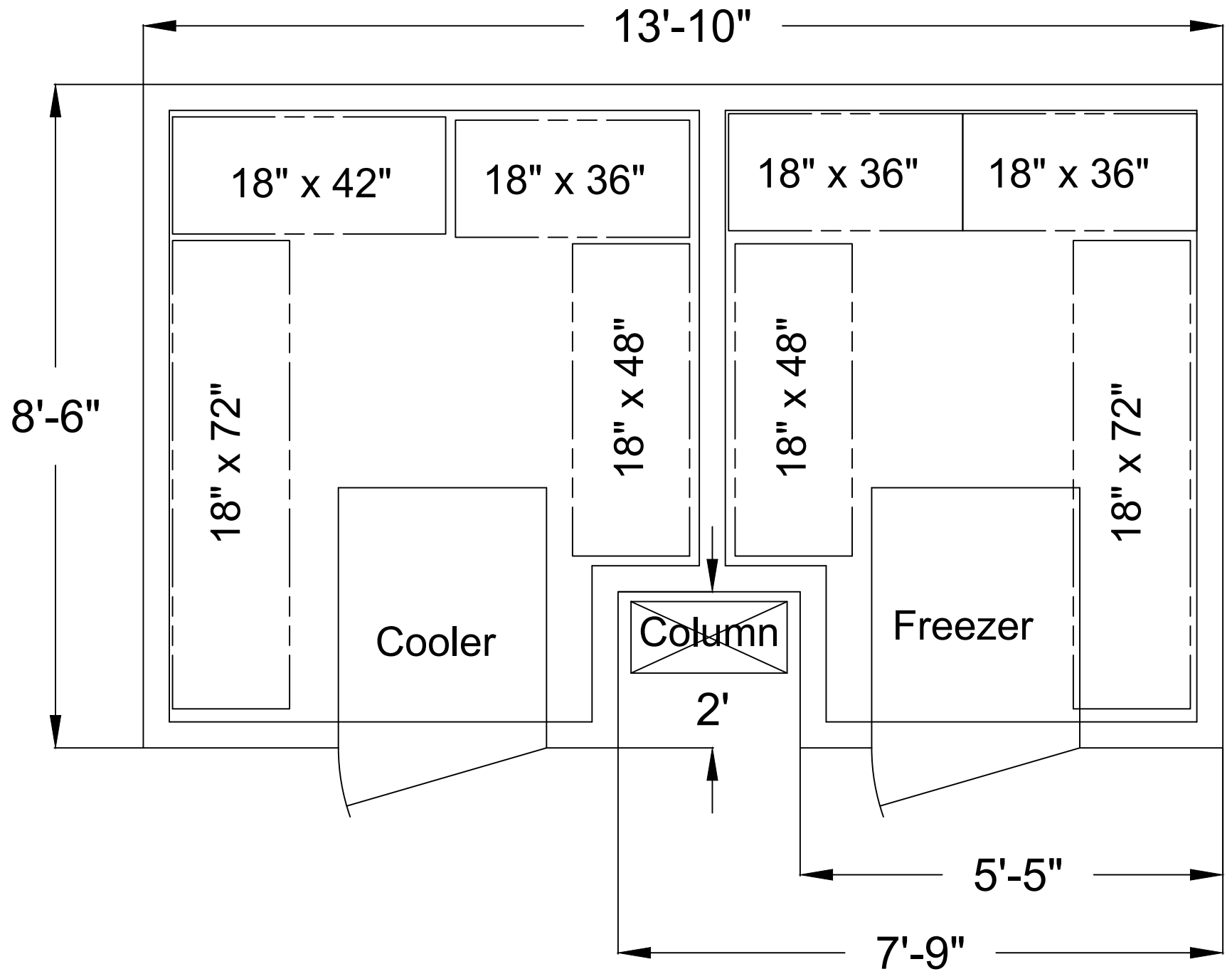
Plan View
